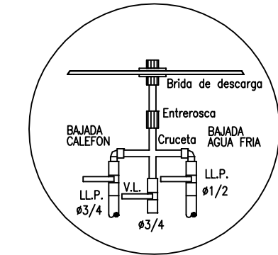
DETALLE COLECTOR
